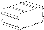
SURE TRACK LARGE BACKER 5 7 / 8 x 6 7 / 8 x 11 5 / 8 " 150 x 175 x 294mm
